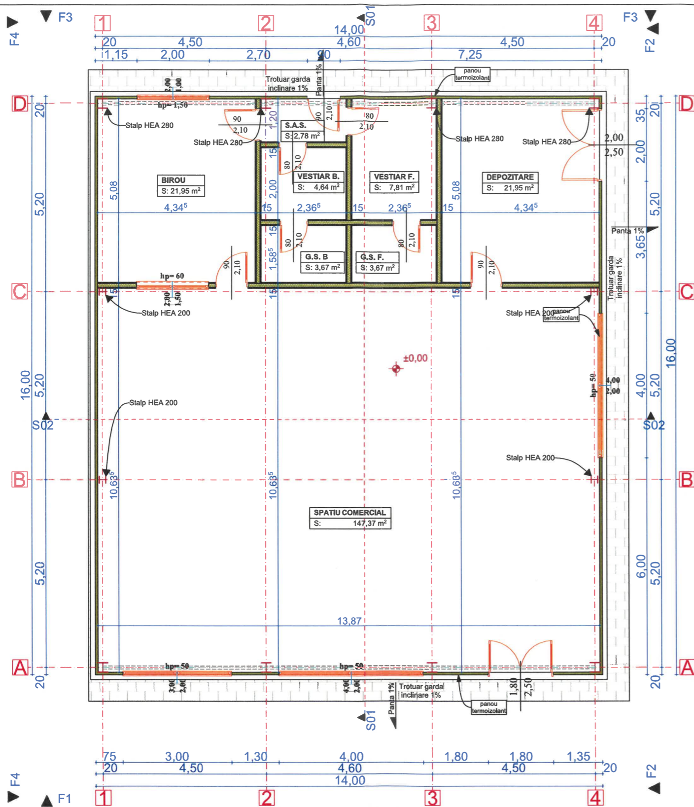
Plan Parter
